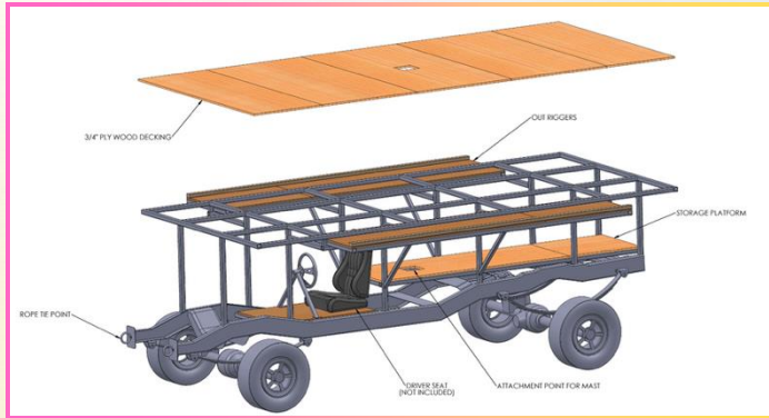
Fabricator's design
